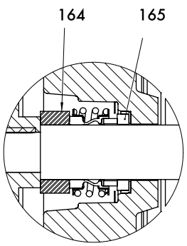
Mechanical Seal Application
