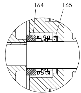
Mechanical Seal Application
