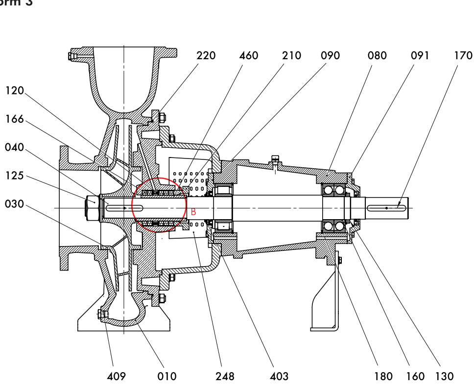
Mechanical Seal Application
